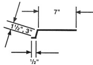
FILLER SHEET (20 GA.) 10'-0" LENGTHS GALVANIZED ONLY
